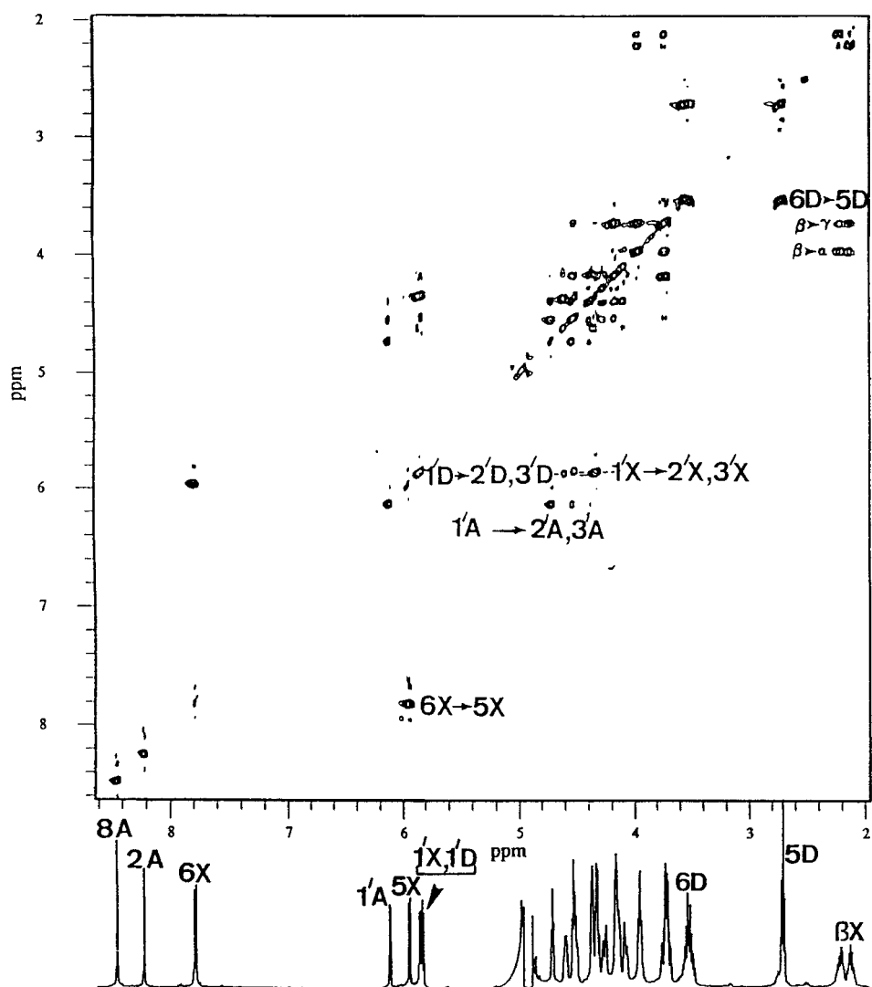
FIG 6A. Two-dimensional homonuclear and heteronuclear correlation spectra of Dp-(acp) 3 UpA in D 2 O. A. The full double quantum filtered COSY spectrum. Some of the assignments are shown on the figure.
