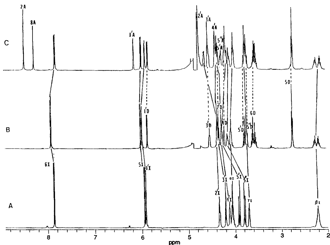
FIG 4. One dimensional ^1\text{H} spectra of the mononucleoside (\text{acp})^3\text{U} ; \text{Dp}-(\text{acp})^3\text{U} ; and \text{Dp}-(\text{acp})^3\text{UpA} . The upfield portions of the ^1\text{H} spectra are shown. The resonances from (\text{acp})^3\text{Up} are labelled X in spectrum A. Numbers refer to positions on the bases, whereas primed numbers refer to positions on the ribose (cf Figure 2 in reference 26). The \alpha , \beta and \gamma refer to positions on the butyric acid side chain of (\text{acp})^3\text{U} , with \alpha referring to the carbon directly bonded to the N-3 of the uridine. Solid lines connect the (\text{acp})^3\text{U} resonances in the spectrum of the monomer (A) to the corresponding resonances in the spectrum of the dimer (B), and trimer (C). The resonances from D in \text{Dp}-(\text{acp})^3\text{U} are labelled with a similar protocol in spectrum B. Dashed lines connect the D resonances in the dimer (B) to that of the trimer (C). The resonances from A in \text{Dp}-(\text{acp})^3\text{UpA} are labelled in spectrum C using the conventional numbering.
