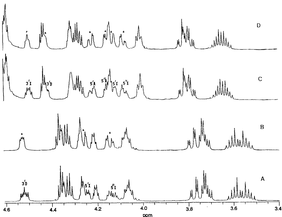
FIG 5. One dimensional ^{31}\text{P} coupled and decoupled, ^1\text{H} spectra of \text{Dp}-(\text{acp})^3\text{U} and \text{Dp}-(\text{acp})^3\text{UpA} . The middle portions of the ^1\text{H} spectra are shown. All four spectra were collected under identical conditions except that spectra B and D included broadband irradiation at the phosphorous frequency as described in the Experimental Section. A and B are the coupled and decoupled spectra of \text{Dp}-(\text{acp})^3\text{U} , respectively; C and D are the coupled and decoupled spectra of \text{Dp}-(\text{acp})^3\text{UpA} , respectively. The resonances from (\text{acp})^3\text{Up} are labelled X in spectra A and C. Stars in spectra B and D specify those multiplets which collapse as a result of disrupted ^{31}\text{P} - ^1\text{H} coupling.
