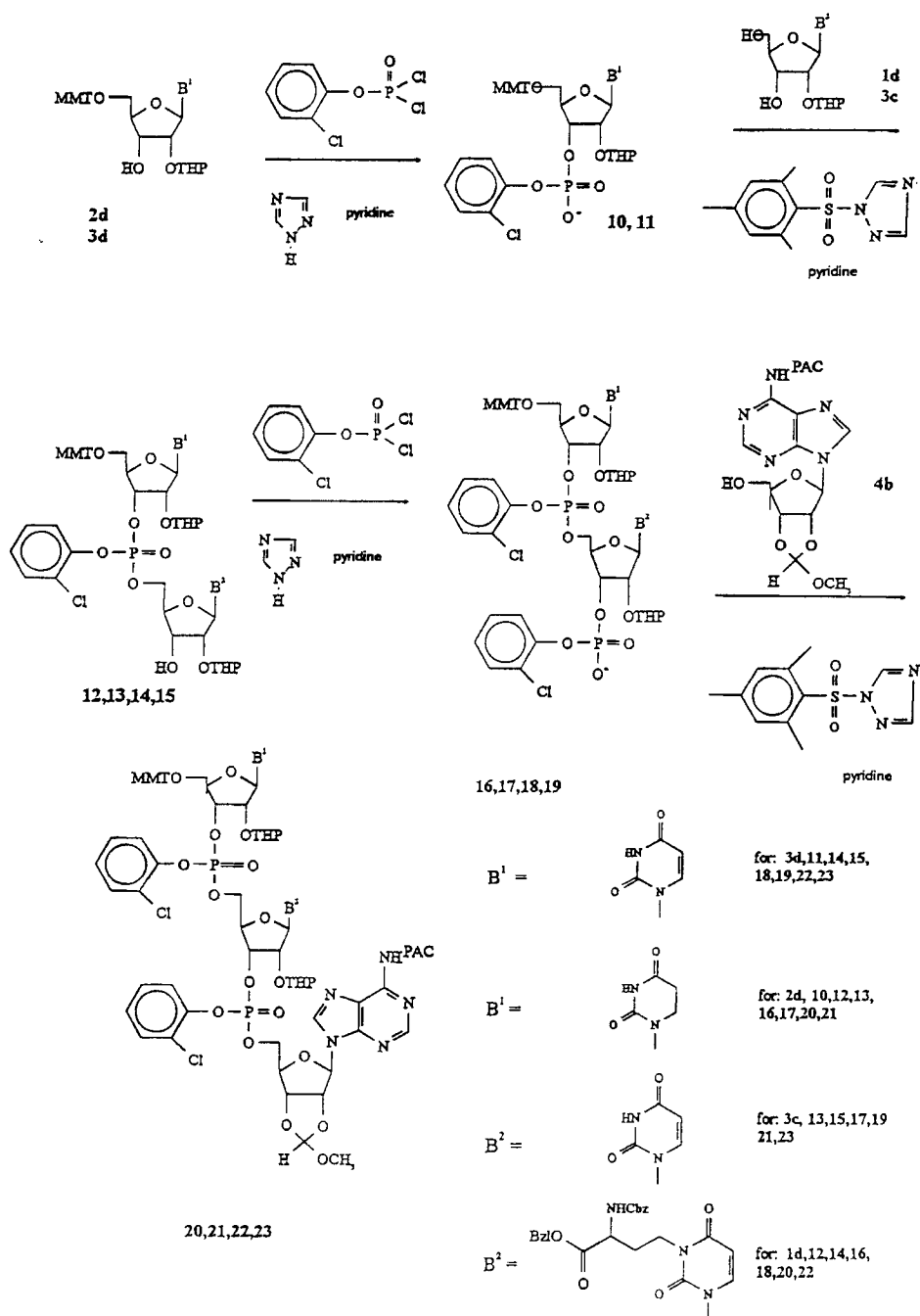
FIG 2. Synthesis of fully protected oligoribonucleotides. The diagram illustrates the synthesis of the fully protected dimer and trimers: Dp-(acp) 3 U, 12; Dp-(acp) 3 UpA, 20; DpUpA, 21; Up-(acp) 3 UpA, 22; and UpUpA, 23.
