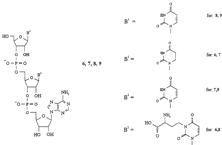
FIG 3. Deprotection of the oligoribonucleotides. The figure depicts the deprotection and molecular structures of the synthesized oligoribonucleotides: Dp-(acp) 3 UpA, 6; DpUpA, 7; Up-(acp) 3 UpA, 8; and UpUpA, 9.
